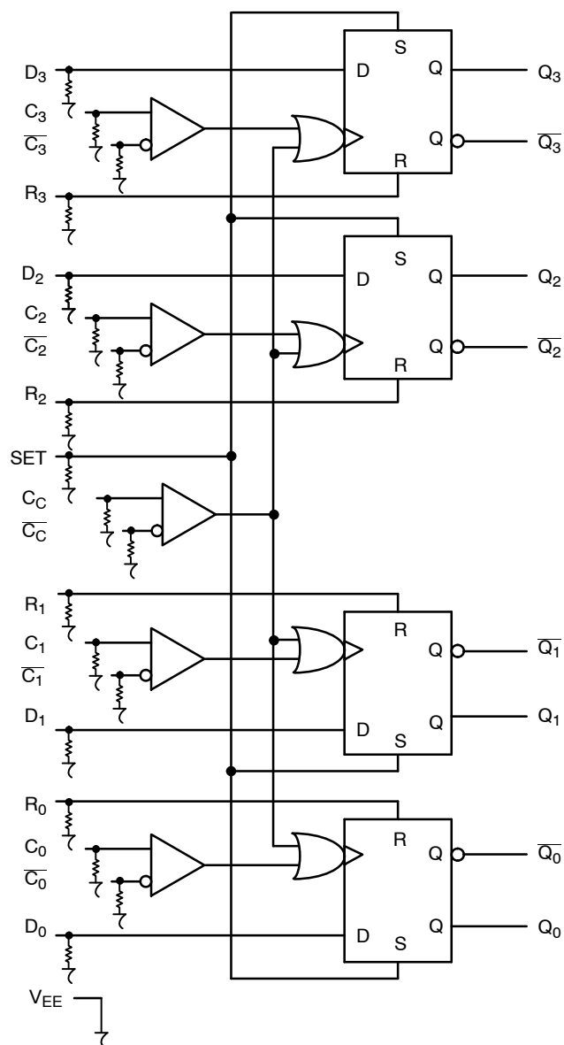
Figure 2. Logic Diagram
