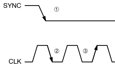
Figure 12. Synchronous Release of SYNC for CKSEL HIGH
