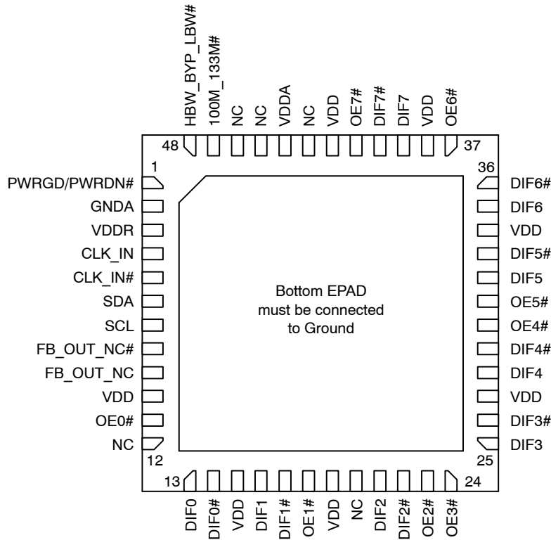
Figure 2. Pin Configuration
