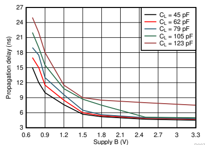
图 6-5. Typical Propagation Delay of Low-to-High (A to B) vs Load Capacitance
