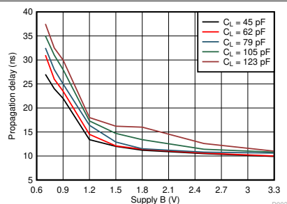
图 6-1. Typical Propagation Delay of Low-to-High (A to B) vs Load Capacitance
