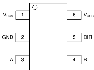
图 4-1. DBV Package 6-Pin SOT-23 (Top View)
