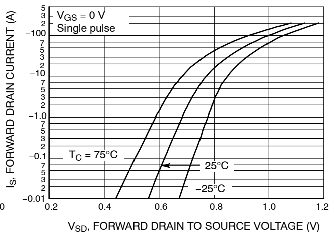
Figure 9. I_S - V_{SD}
