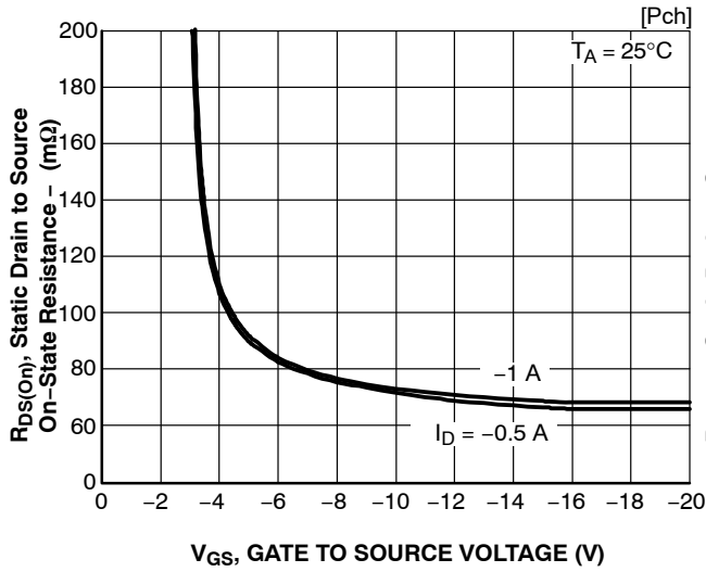
Figure 14. R_{DS(on)} - V_{GS}
