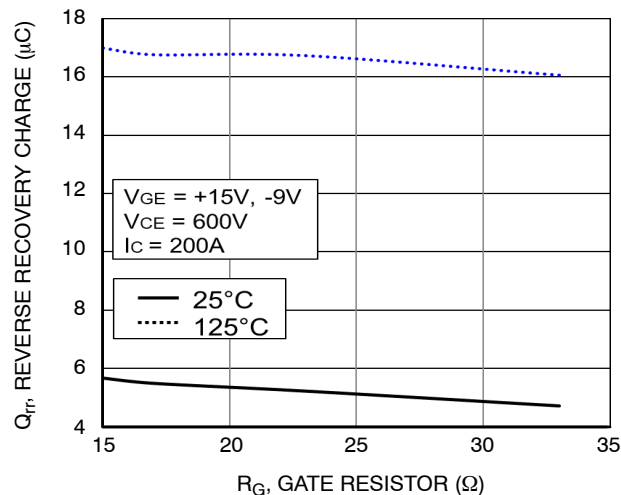
Figure 56. Typical Reverse Recovery Charge vs. R_G
