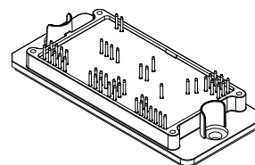
Q2PACK POSITIVE SOLDER PINS CASE 180HH
