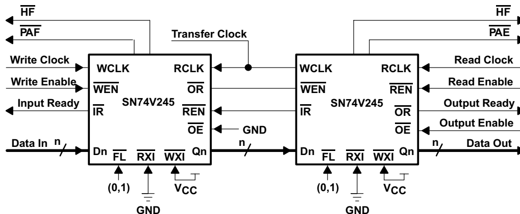
Figure 29. Block Diagram of 8192 × 18 Synchronous FIFO Memory With Programmable Flags Used in Depth-Expansion Configuration
