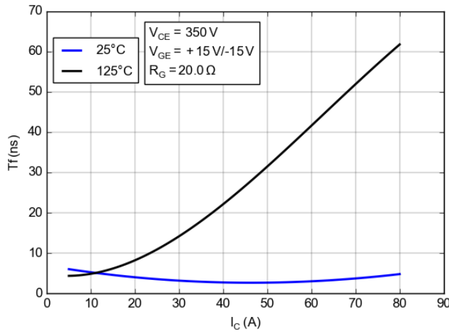
Figure 50. Typical Switching Times Tf vs. I_C
