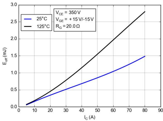
Figure 42. Typical Turn Off Loss vs. I_C
