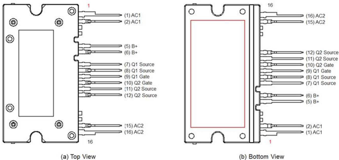
Figure 1. Pin Configuration
