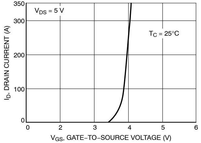
Figure 12. Transfer Characteristics
