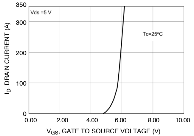
Figure 12. Transfer Characteristics
