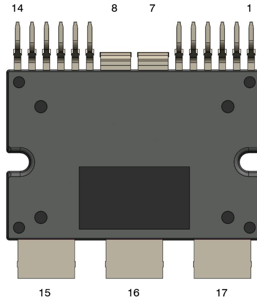
Figure 1. Pin Configuration
