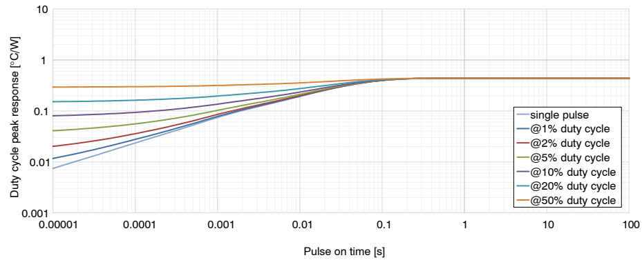
Figure 26. Diode Transient Thermal Impedance
