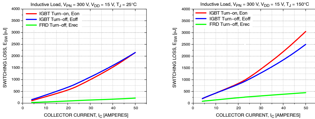
Figure 5. Switching Loss Characteristics
