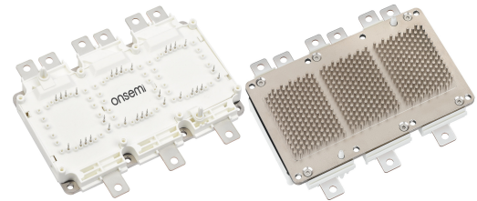
SSDC39 154.40x92.0 (SPB) CASE 183AM
