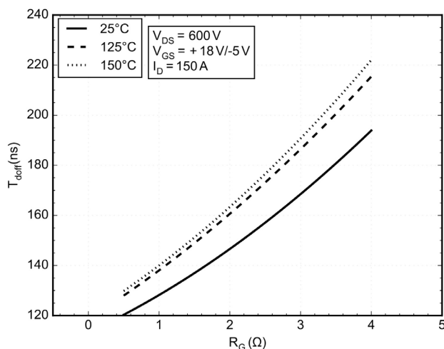
Figure 15. Typical Switching Loss Tdoff vs. Rg
