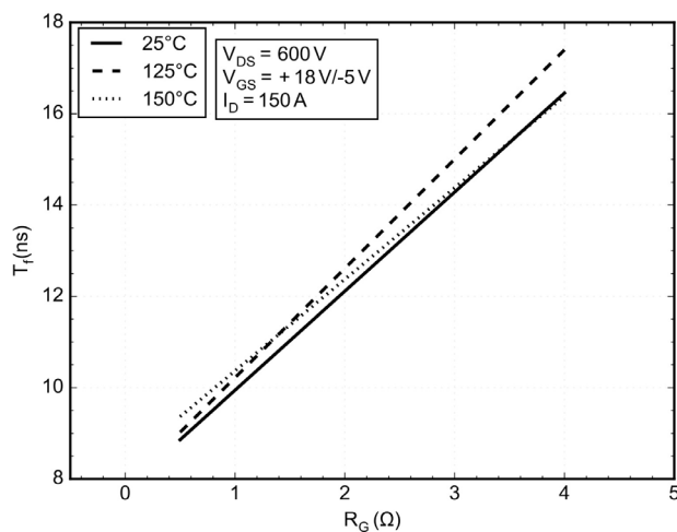
Figure 19. Typical Switching Loss Tf vs. Rg
