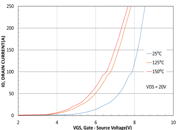
Figure 5. MOSFET Typical Transfer Characteristics
