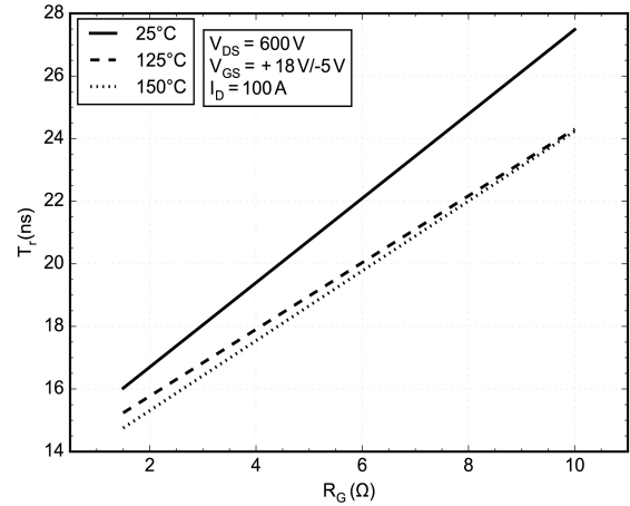
Figure 18. Typical Turn-On Switching T_r vs. R_G
