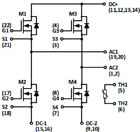
Figure 1. NXH030F120M3F1PTG Schematic Diagram
