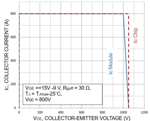
Figure 7. RBSOA
