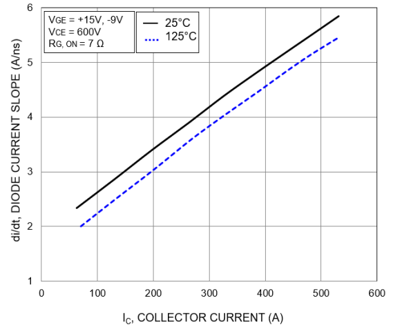
Figure 37. Typical di/dt vs. I_c
