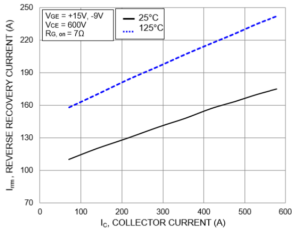
Figure 54. Typical Reverse Recovery Current vs. I_c
