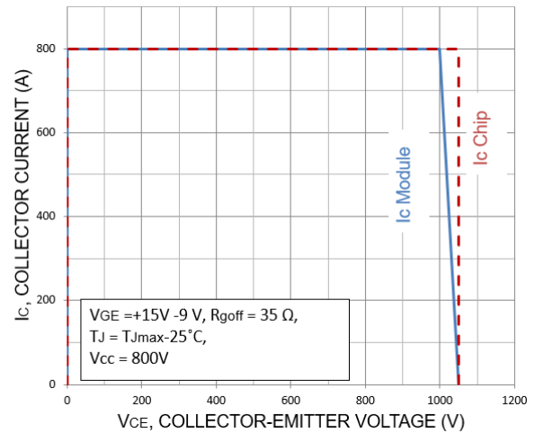
Figure 16. RBSOA
