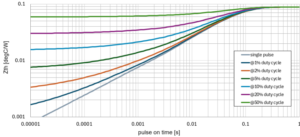
Figure 19. Transient Thermal Impedance (IGBT Z_{thjc} )
