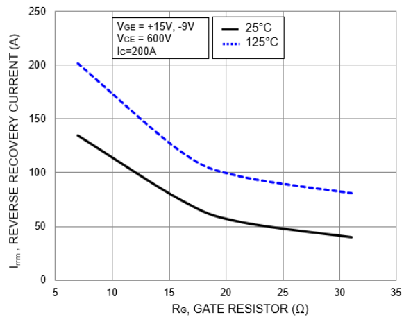
Figure 58. Typical Reverse Recovery Peak Current vs. R_G
