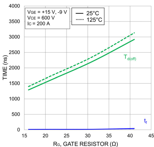
Figure 48. Typical Turn-Off Switching Time vs. R_G
