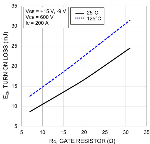
Figure 44. Typical Turn On Loss vs. R_G
