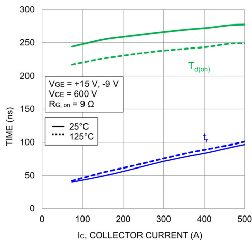
Figure 29. Typical Turn-On Switching Time vs. I_C
