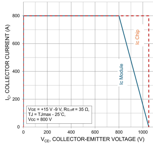
Figure 16. RBSOA
