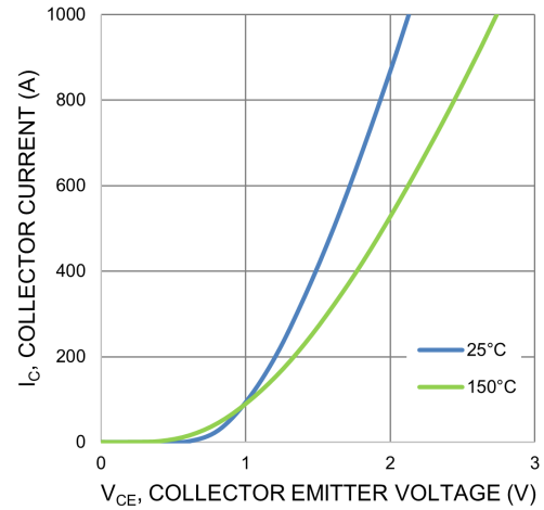
Figure 14. Saturation Voltage Characteristic – IGBT
