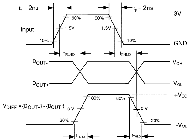
Figure 3. AC Waveforms
