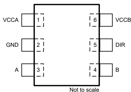
图 4-2. DCK Package, 6-Pin SOT-SC70 (Top View)
