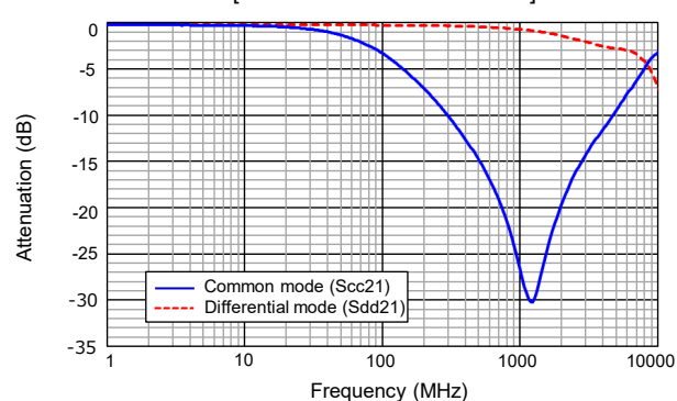
[ Attenuation characteristics ]
