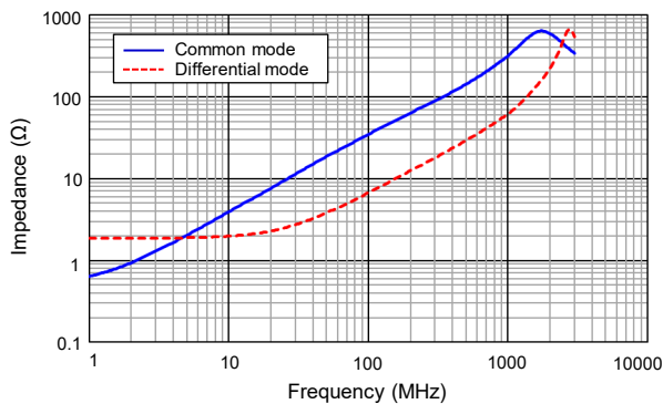
[ Impedance characteristics ]
