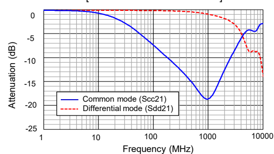
[ Attenuation characteristics ]
