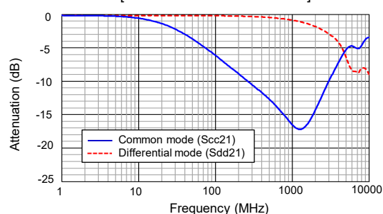
[ Attenuation characteristics ]
