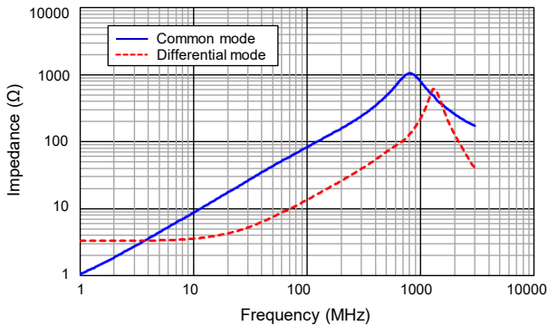
[ Impedance characteristics ]
