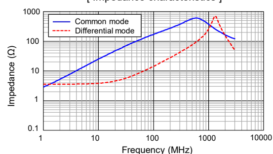
[ Impedance characteristics ]
