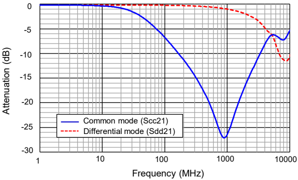
[ Attenuation characteristics ]
