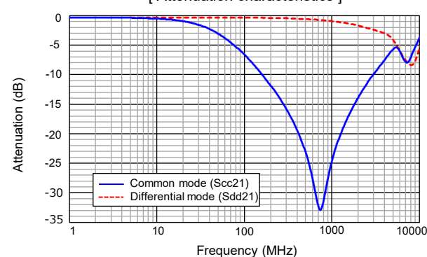
[ Attenuation characteristics ]
