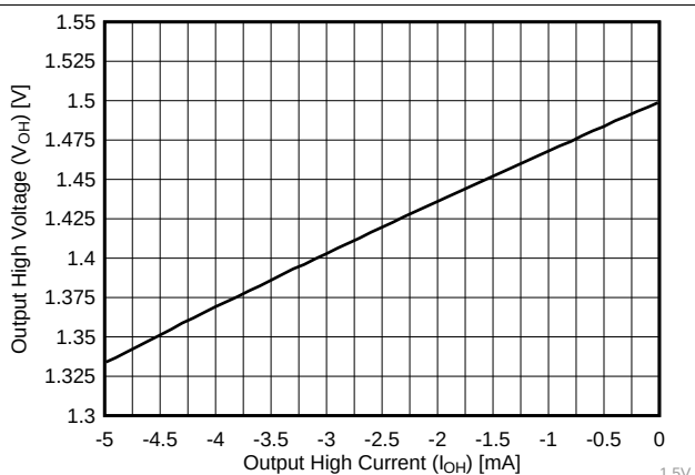
图 6. Typical Output High Voltage of 1.5 V (25°C)
