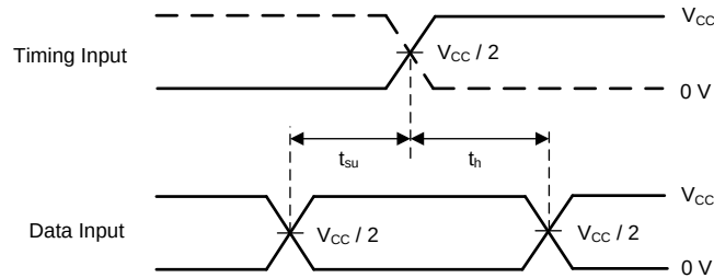
图 12. Voltage Waveforms: Setup and Hold Times
