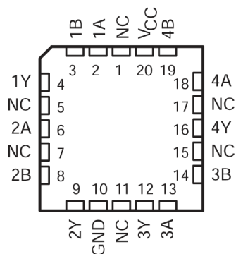
NC – No internal connection Figure 3-2. SN54ACT86 FK Package (Top View)
