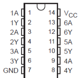
图 5-1. SN54ACT04 J or W Package; SN74ACT04 D, DB, N, NS, or PW Package Top View
