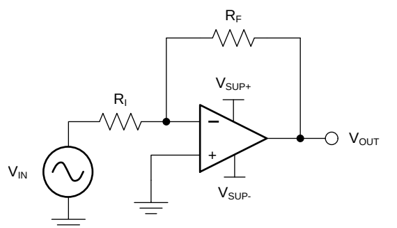
Figure 15. Application Schematic
