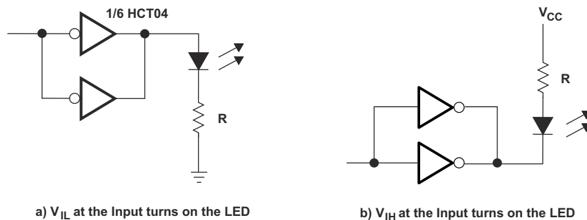
图 8-2. Driving LEDs
