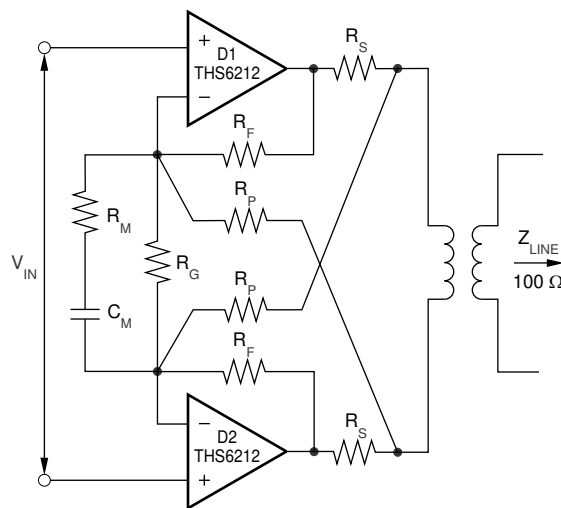
图 7-7. 0.1-dB Flatness Compensation Circuit
