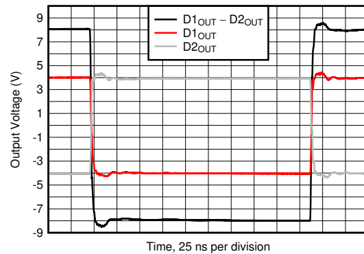
图 5-26. Large-Signal Pulse Response
