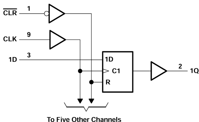
图 8-1. Logic Diagram (Positive Logic)
