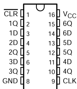
图 5-1. Package SN74AHCT174 D, DB, DGV, N, NS, or PW Package (Top View)
