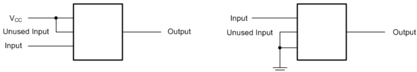
图 9-1. Layout Recommendation
