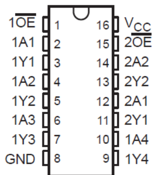
图 5-1. D, DB, DGV, N, or PW Package (Top View)
