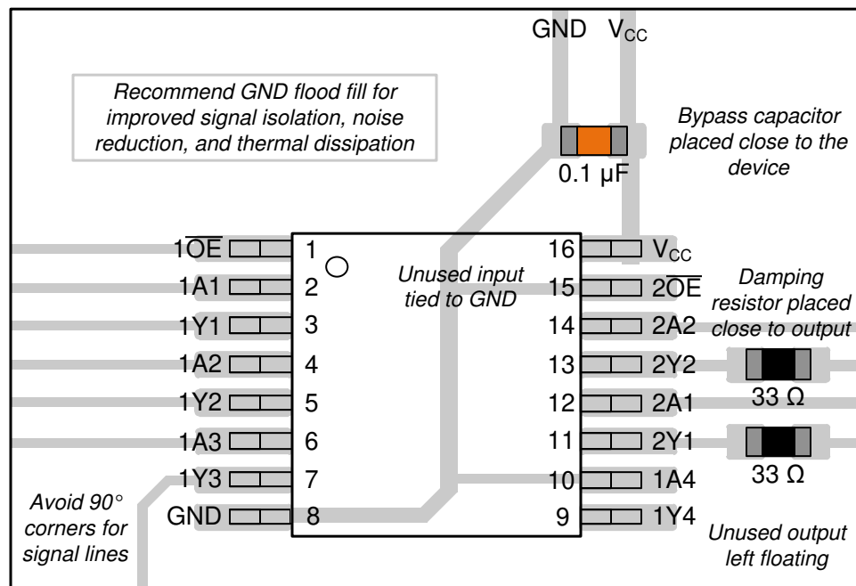
图 9-2. Example Layout for the SN74AHC367
