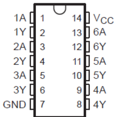
图 4-1. CD54AC04 F Package, CD74AC04 E or M Package, Top View
