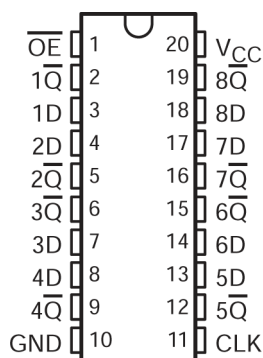
图 3-1. SN74AC534 DB, DW, N, NS, or PW Package (Top View)
