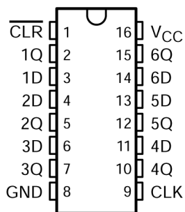
图 4-1. CD54ACT174 J Package, 16-PIN CDIP; CD74ACT174 N or D Package, 16-PIN PDIP or SOIC (Top View)
