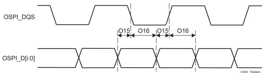
图 7-94. OSPI0 Timing Requirements – PHY Data Training, DDR with DQS
