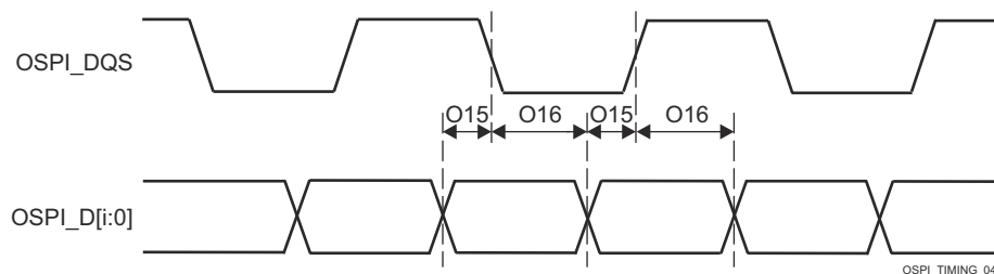
图 7-101. OSPI0 Timing Requirements – PHY DDR with External Board Loopback or DQS
