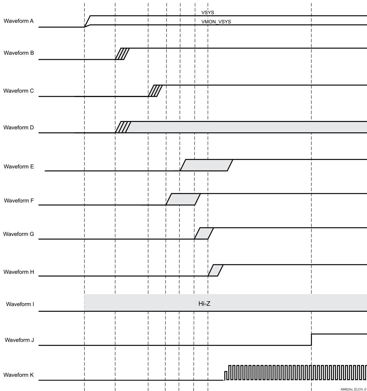
图 7-5. Power-Up Sequencing
