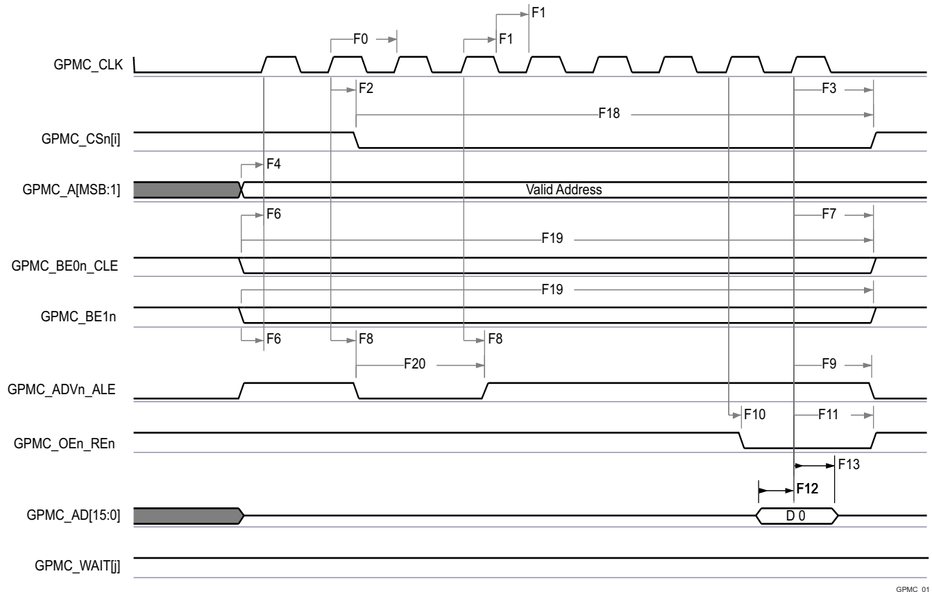
图 7-46. GPMC and NOR Flash — Synchronous Single Read (GPMCFCLKDIVIDER = 0)
