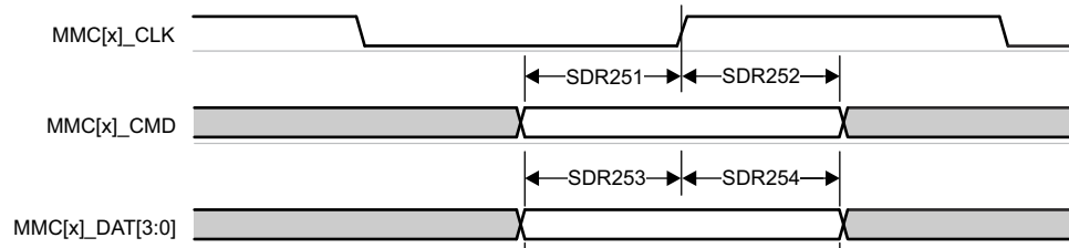
图 7-89. MMC1/MMC2 - UHS-I SDR25 - Receive Mode
