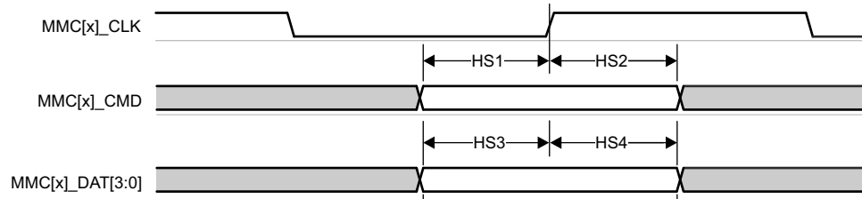
图 7-85. MMC1/MMC2 - High Speed - Receive Mode
