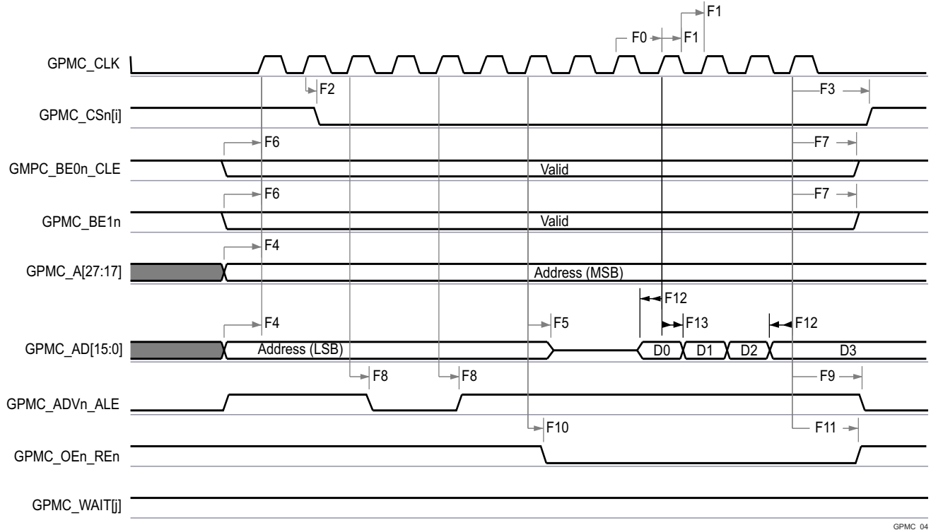
图 7-48. GPMC and NOR Flash—Synchronous Burst Write (GPMCFCLKDIVIDER = 0)
