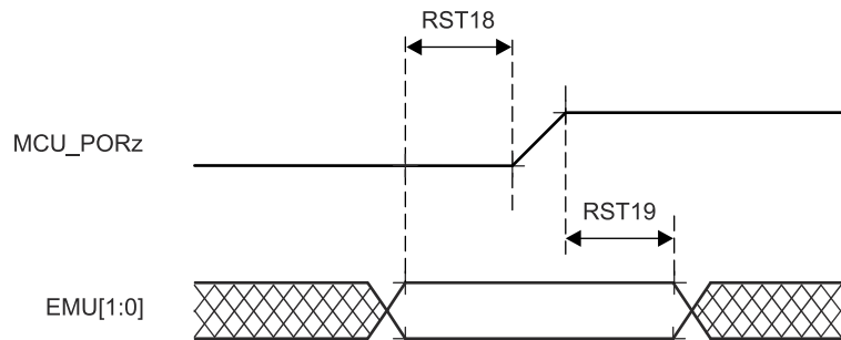
图 7-11. EMUx Timing Requirements
