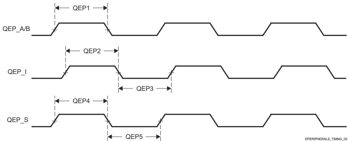
图 7-45. EQEP Timing Requirements
