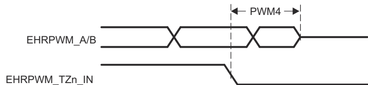
图 7-44. EHRPWM_TZn_IN to EHRPWM_A/B Hi-Z Switching Characteristics
