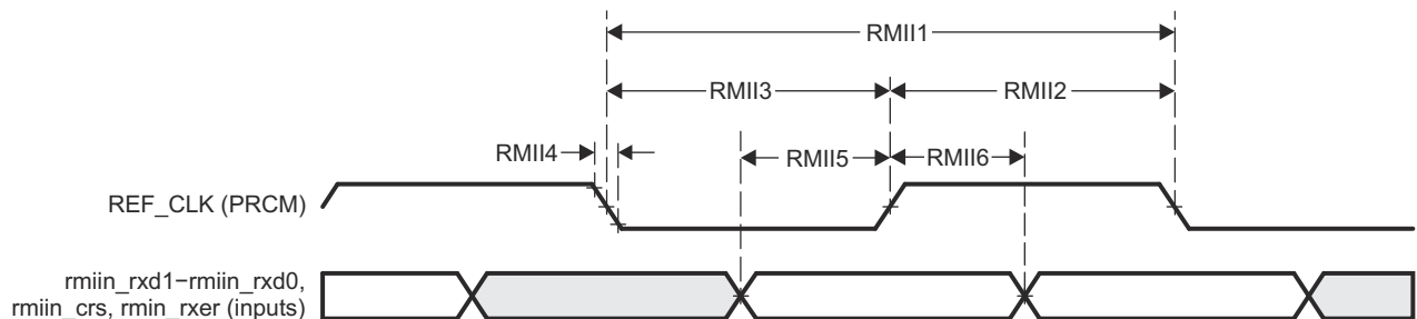
图 6-14. GMAC Receive Interface Timing RMII In operation
