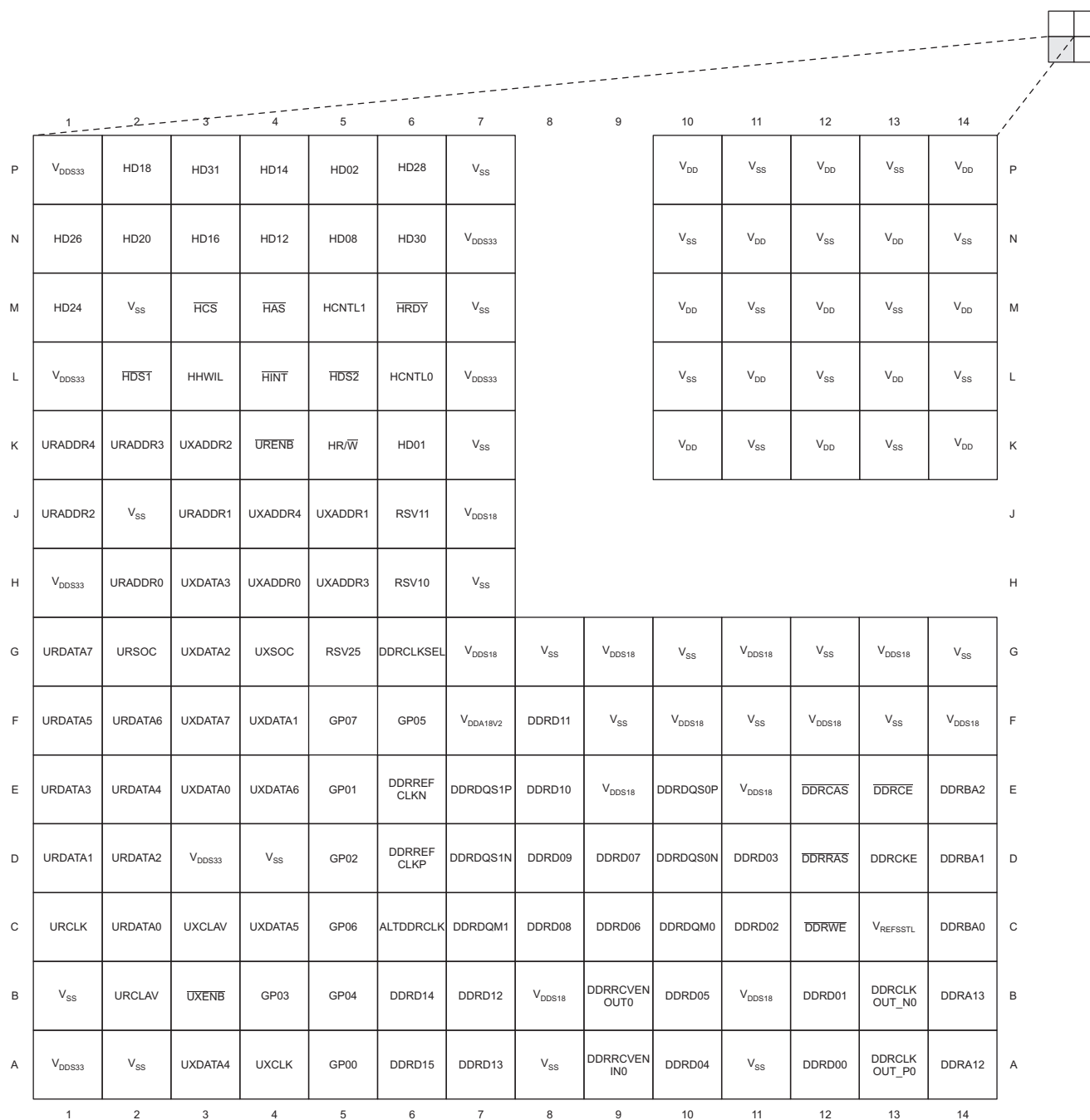
Figure 3-5. TCI648F Pin Map (Bottom View) [Quadrant D]
