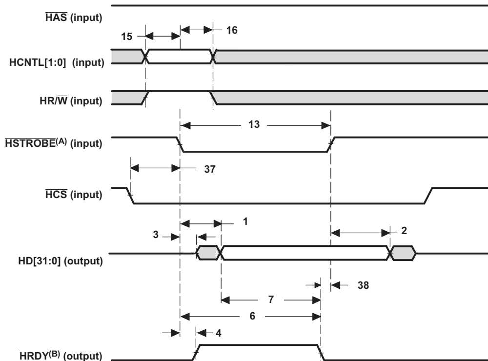
Figure 4-47. HPI32 Read Timing ( \overline{HAS} Not Used, Tied High)
