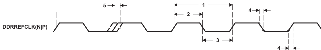
Figure 4-30. DDRREFCLK(N|P) Timing
