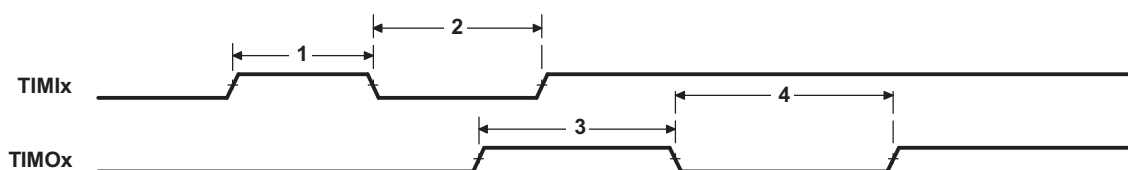
Figure 4-61. Timer Timing
