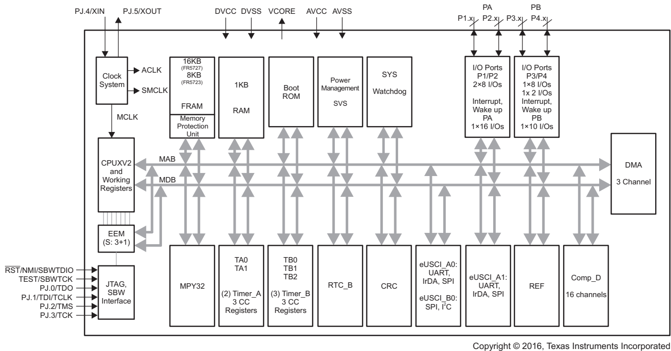
图 6-2. Functional Block Diagram – RHA Package – MSP430FR5723, MSP430FR5727
