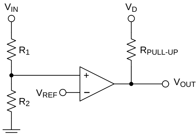
Figure 24. Threshold Detector
