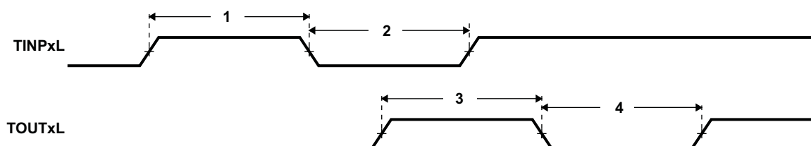
Figure 6-43. Timer Timing
