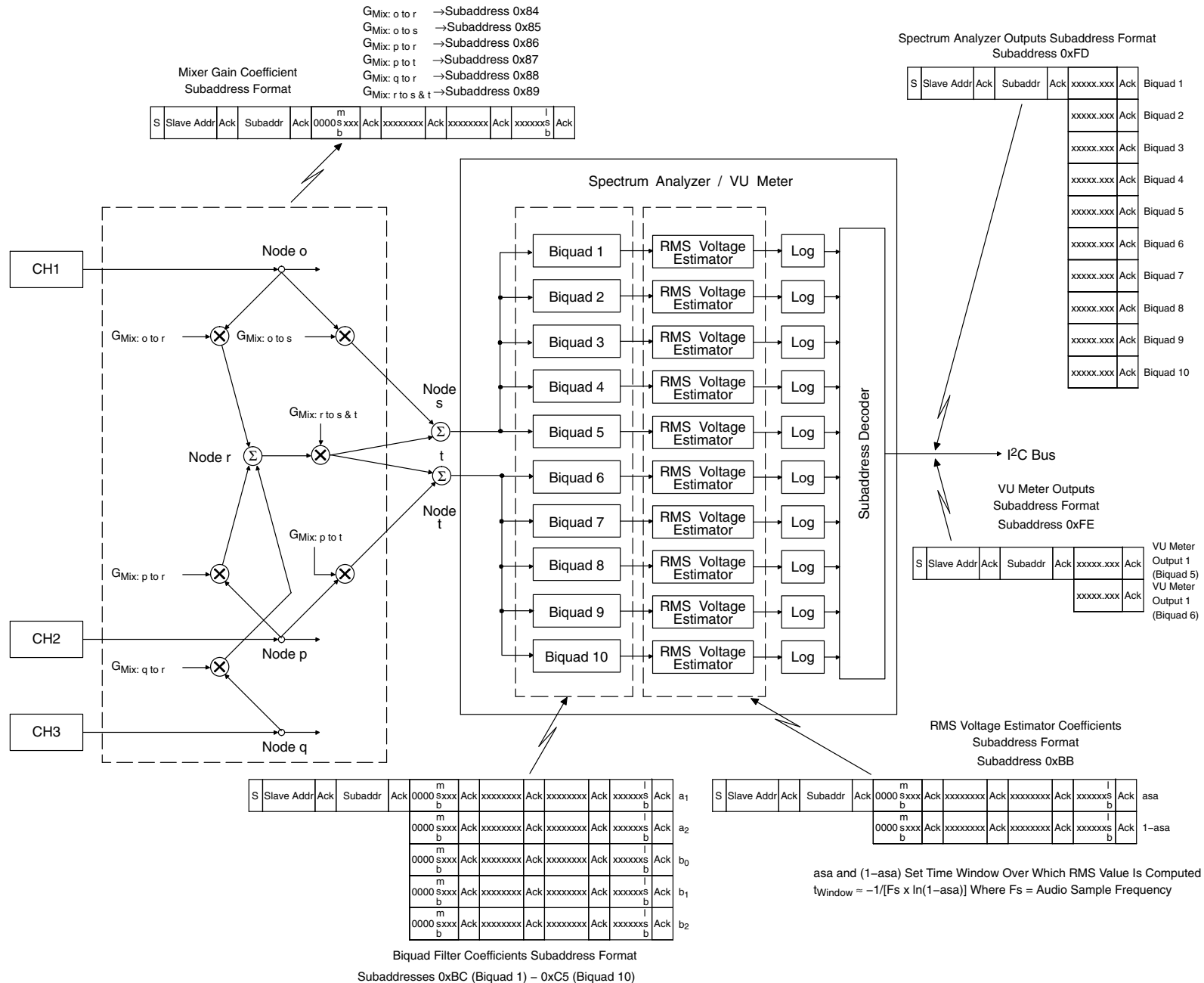
Figure 3-29. Spectrum Analyzer/VU Meter Block Diagram
