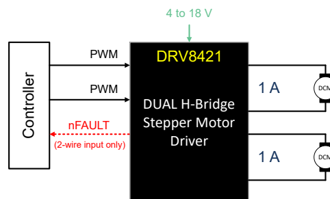
Simplified Schematic
