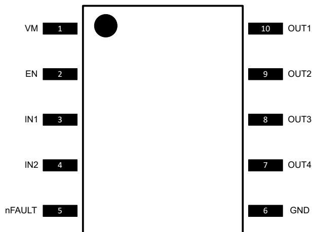
Figure 5-4. DRV8421B 10-Pin SSOP Top View
