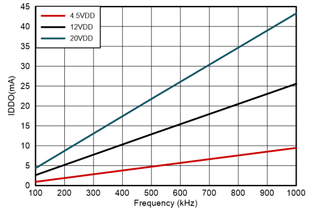
图 6-4. Operating Supply Current (both outputs switching)
