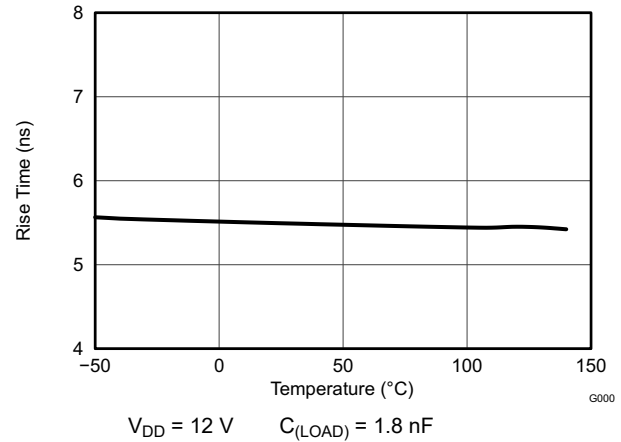
图 5-12. Rise Time vs Temperature
