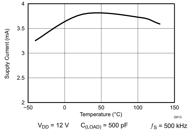
图 5-6. Operating Supply Current vs Temperature (Output Switching)
