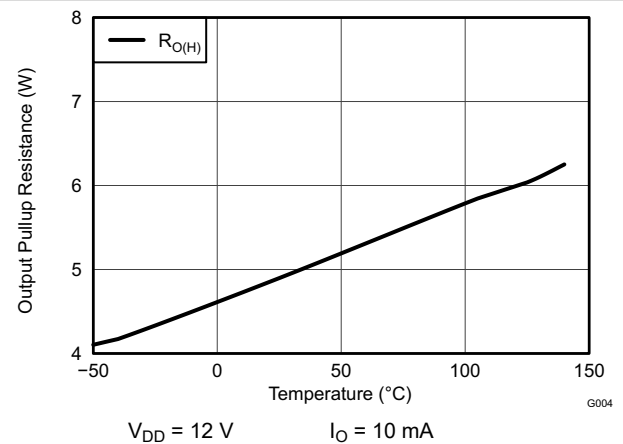
图 5-10. Output Pullup Resistance vs Temperature
