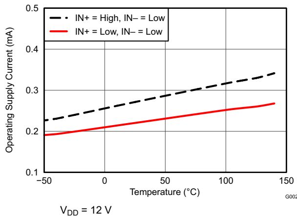
图 5-7. Supply Current vs Temperature (Output in DC On or Off Condition)
