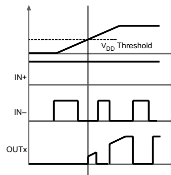
图 6-2. Power-Up (Inverting Drive)
