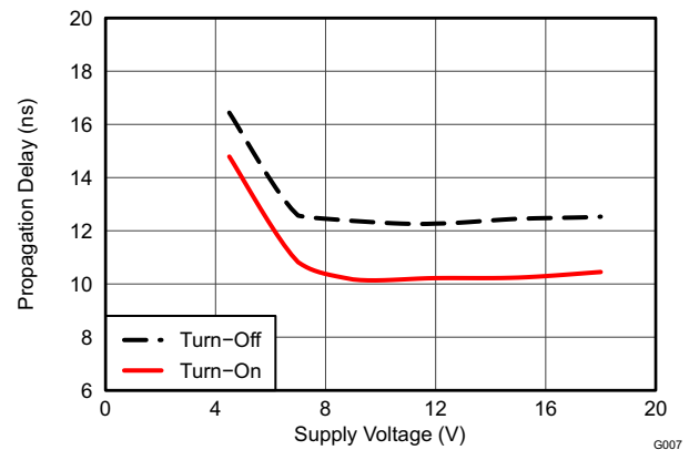
图 5-16. Propagation Delays vs Supply Voltage
