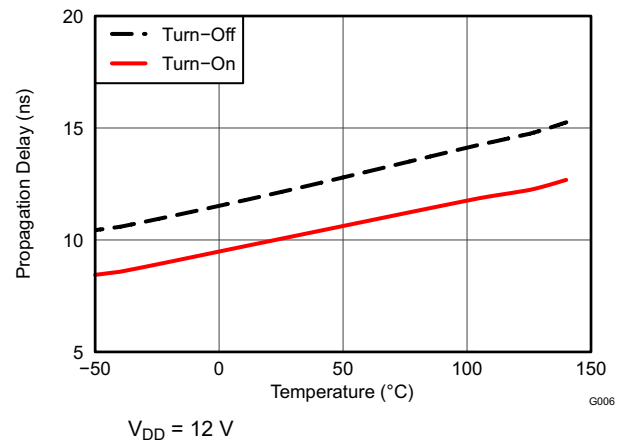
图 5-14. Input to Output Propagation Delay vs Temperature
