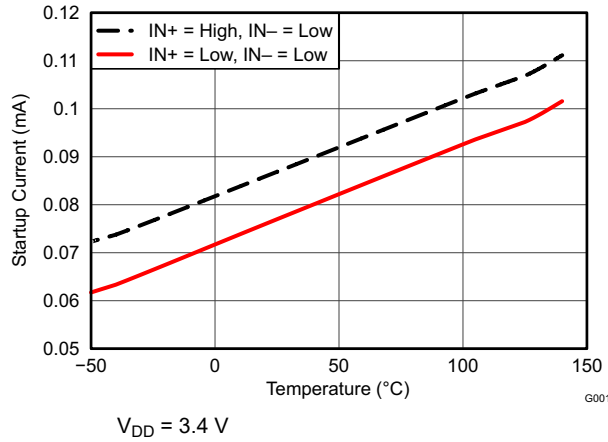
图 5-5. Startup Current vs Temperature
