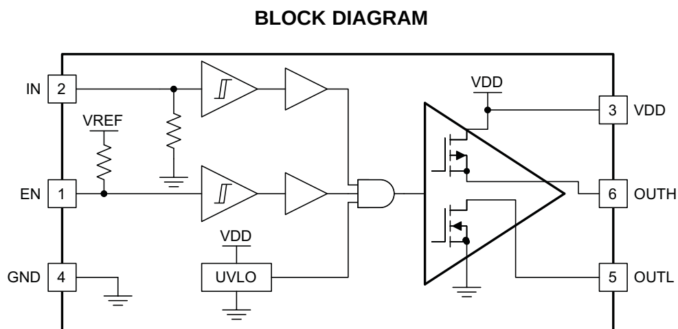
Figure 2. UCC27531-Q1 (EN Pullup Resistance to VREF = 500 k \Omega , VREF = 5.8 V, in Pulldown Resistance to GND = 230 k \Omega )
