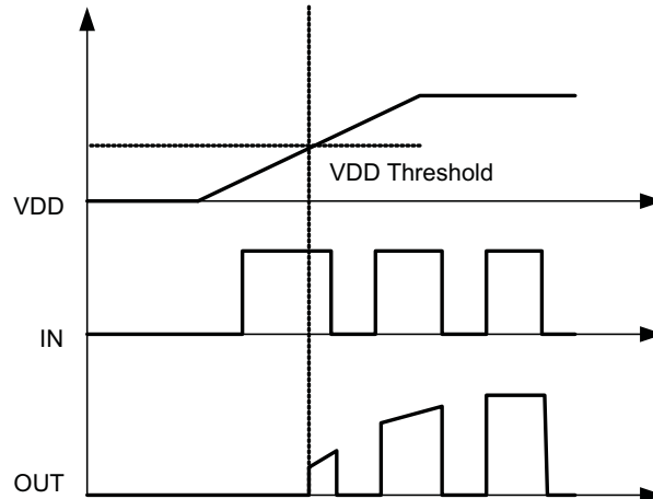
Figure 26. Power Up
