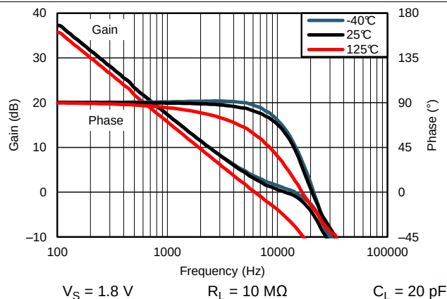
Figure 35. Gain and Phase vs Temperature at 1.8 V
