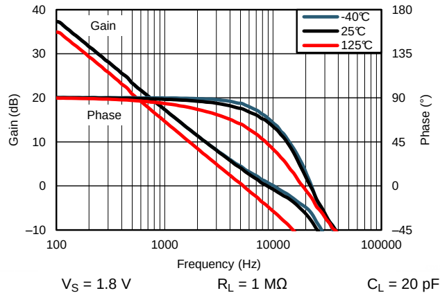
Figure 33. Gain and Phase vs Temperature at 1.8 V
