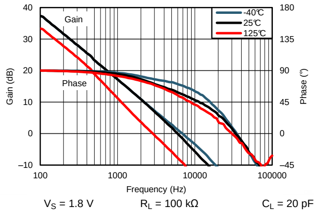
Figure 31. Gain and Phase vs Temperature at 1.8 V
