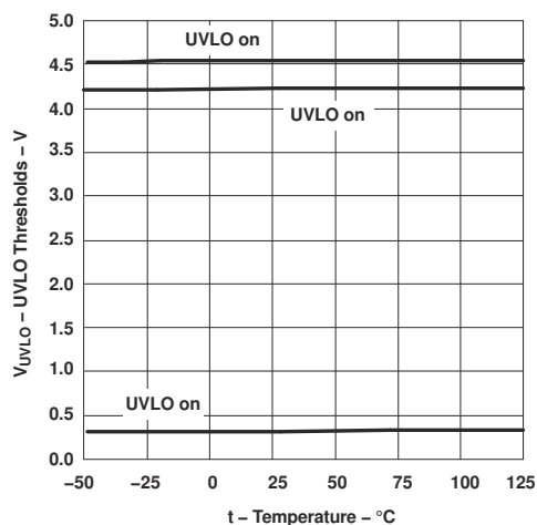
图 8-2. UVLO Thresholds vs Temperature
