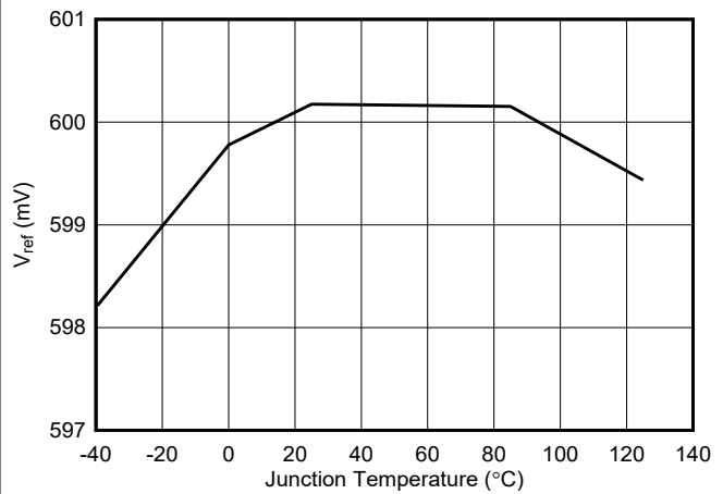
Figure 5-2. Vref Voltage
