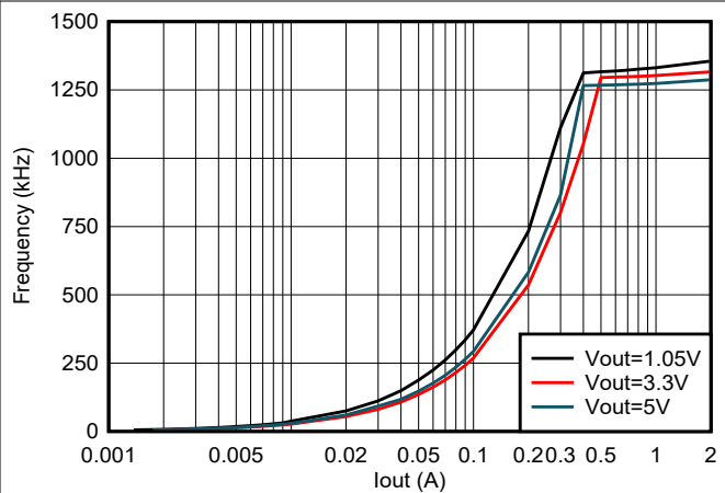
Figure 5-8. TPS562243 Frequency vs Loading
