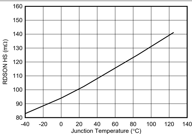
Figure 5-5. Low-Side Rdson
