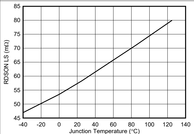
Figure 5-6. High-Side Rdson
